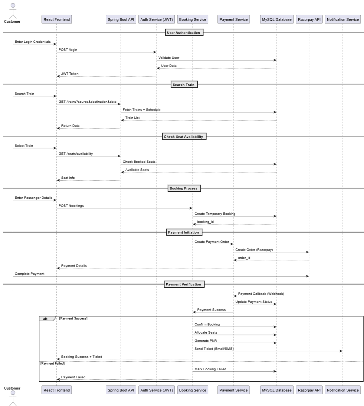
Fig 3 : Sequence Diagram
